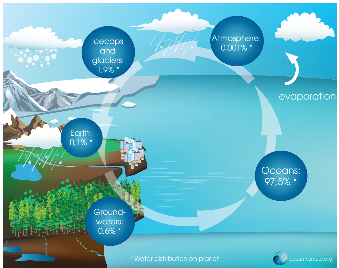
Water cycle
